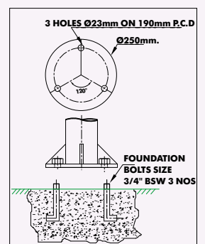
Installation Schematics
