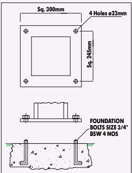
Installation Schematics
