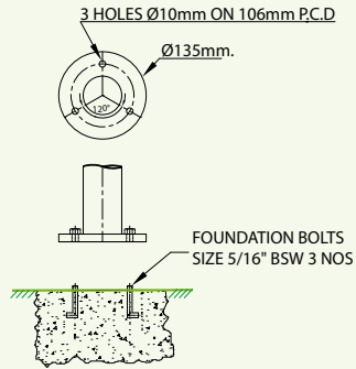
Installation Schematics
