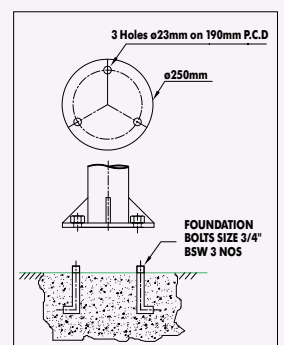
Installation Schematics
