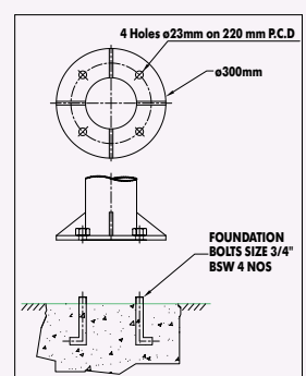
Installation Schematics
