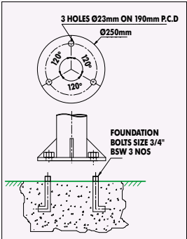
Installation Schematics
