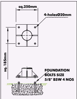
Installation Schematics
